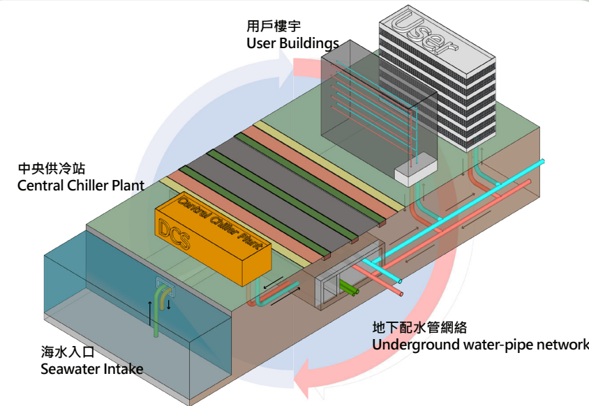
區域供冷系統網絡 Network of District Cooling System
