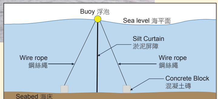
淤泥屏障橫切面圖 Cross section of Silt curtain
